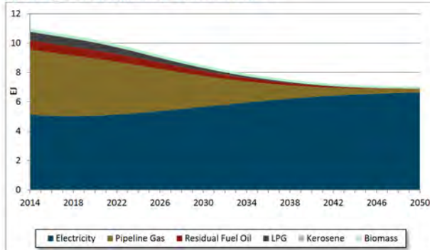
Figure 13. Residential Energy Demand, All Decarbonization Cases
