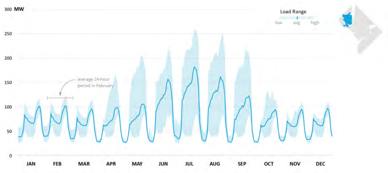
Figure 9: 2032 Scenario 1 electric load profiles for substation 129.
