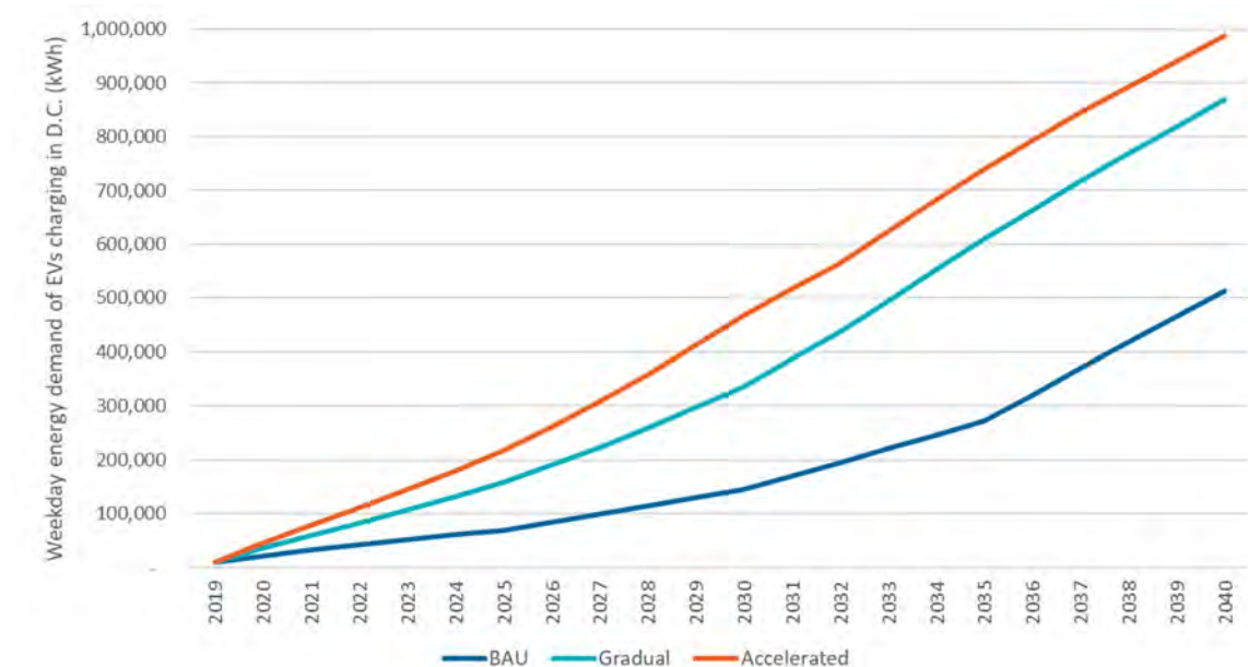
Figure 21 Total energy demand
