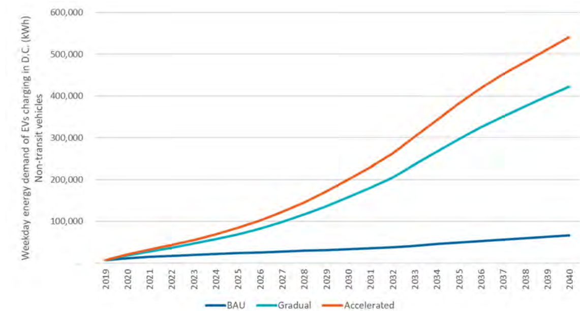
Figure 19 Non-transit Energy Demand in Three Scenarios (2020-2040)
