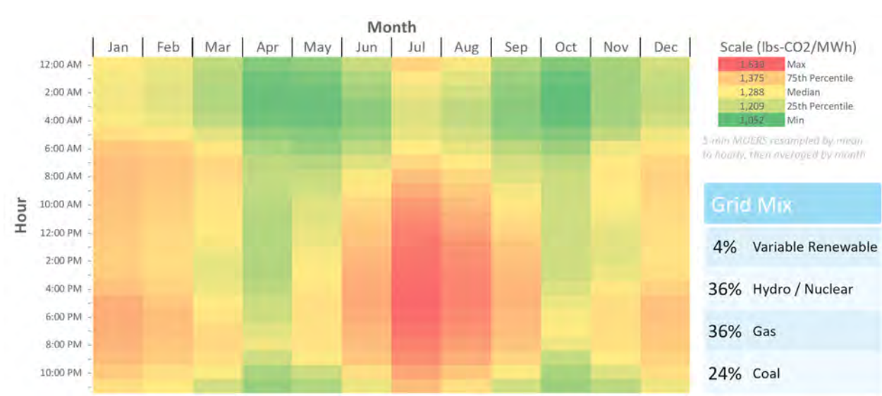
Figure 33: 2019 PJM Atlantic MOER data heat map.
