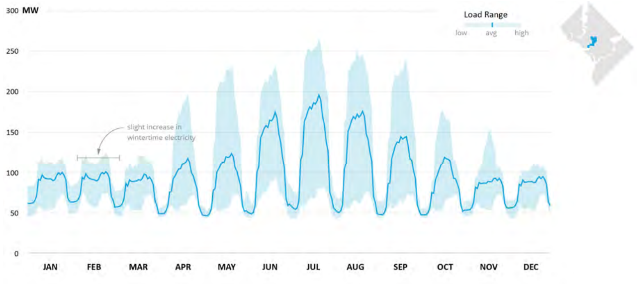
Figure 8: 2032 Scenario 1 electric load profiles for substation 52.
