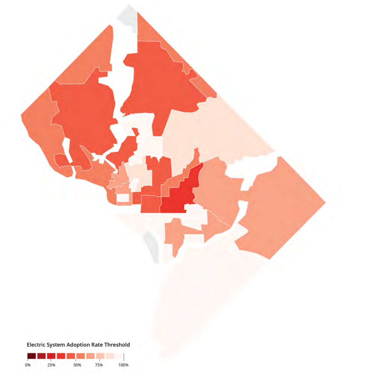
Figure 12: Threshold adoption rates for electrification by substation zone
