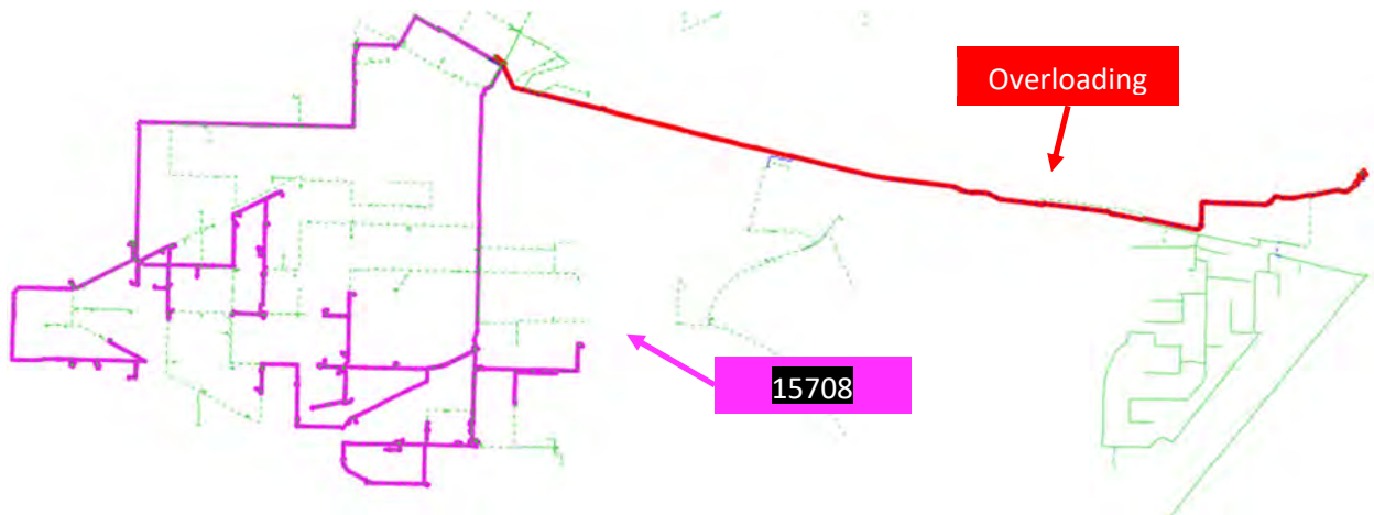
Figure A.15: Loading violation of Feeder 15708 under normal condition in 2032 with electrification and EV impact
