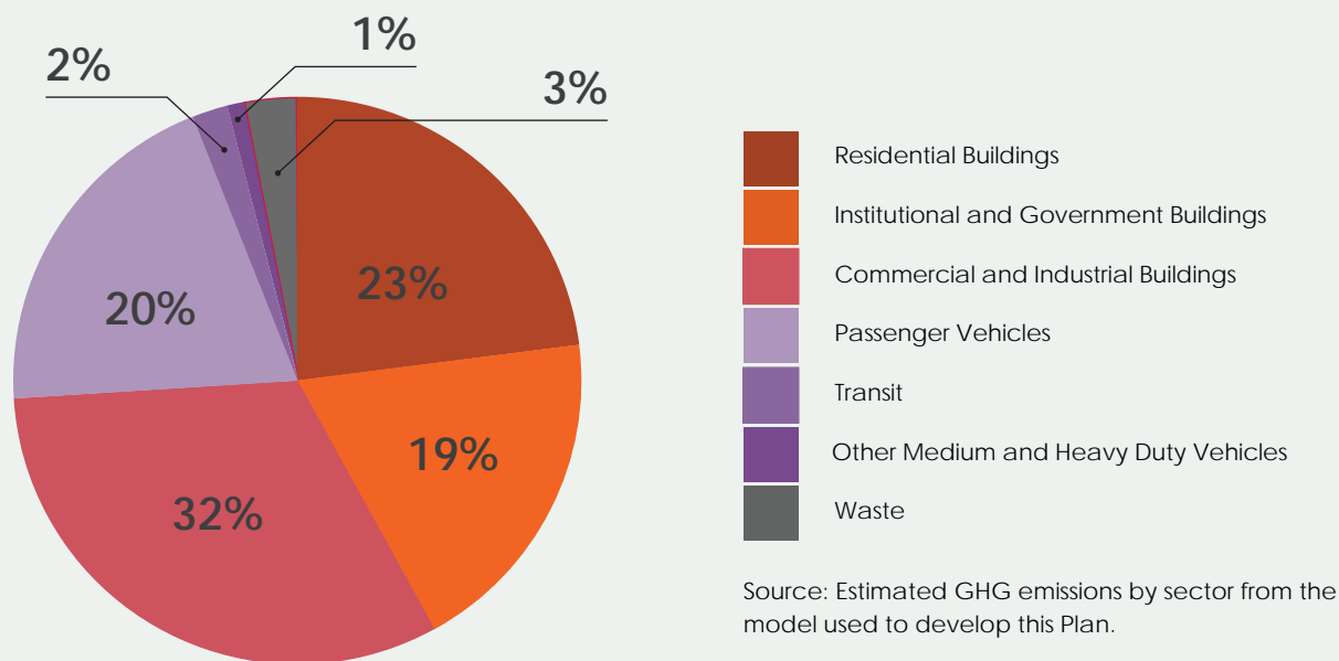
▼ Figure 4: Modeled proportion of GHG emissions by sector, 2015
