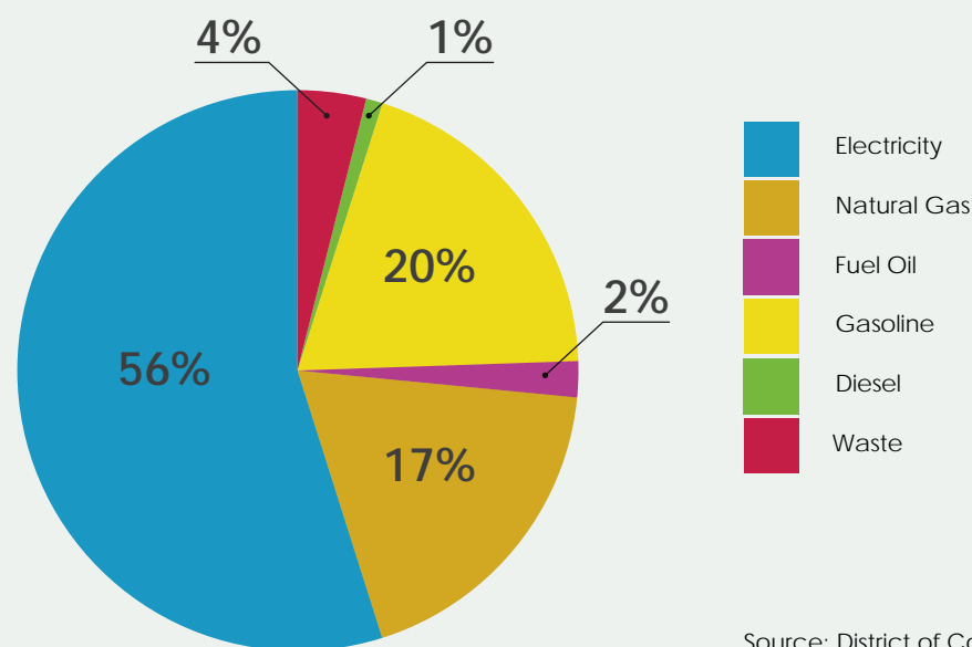
▼ Figure 5: Proportion of GHG emissions by source, 2012
