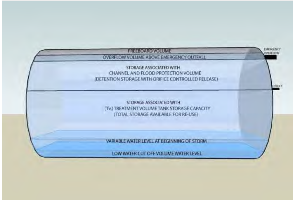
Figure 3.8 Incremental design volumes associated with tank sizing.
