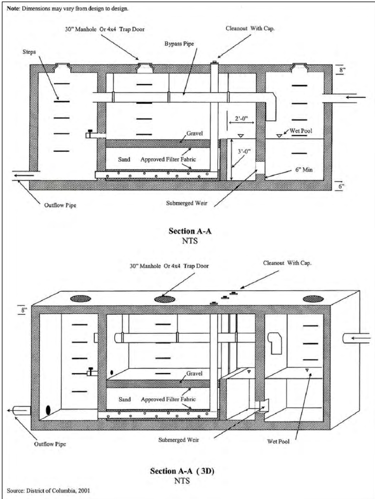
Figure 3.23 Example of a three-chamber underground sand filter (F-3) for separate sewer areas. Note: Material specifications are indicated in Table 3.28.
