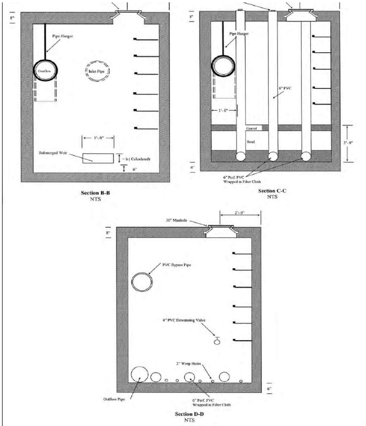
Figure 3.24 Example of a three-chamber underground sand filter (F-3) for separate sewer areas. Note: Material specifications are indicated in Table 3.28.
