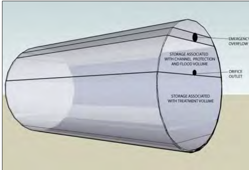
Figure 3.6 Tank Design 2: Storage associated with design storm, channel protection, and flood volume.
