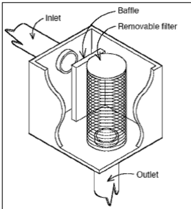
Figure 3.4 Diagram of a roof washer. (TWRB, 2005)
