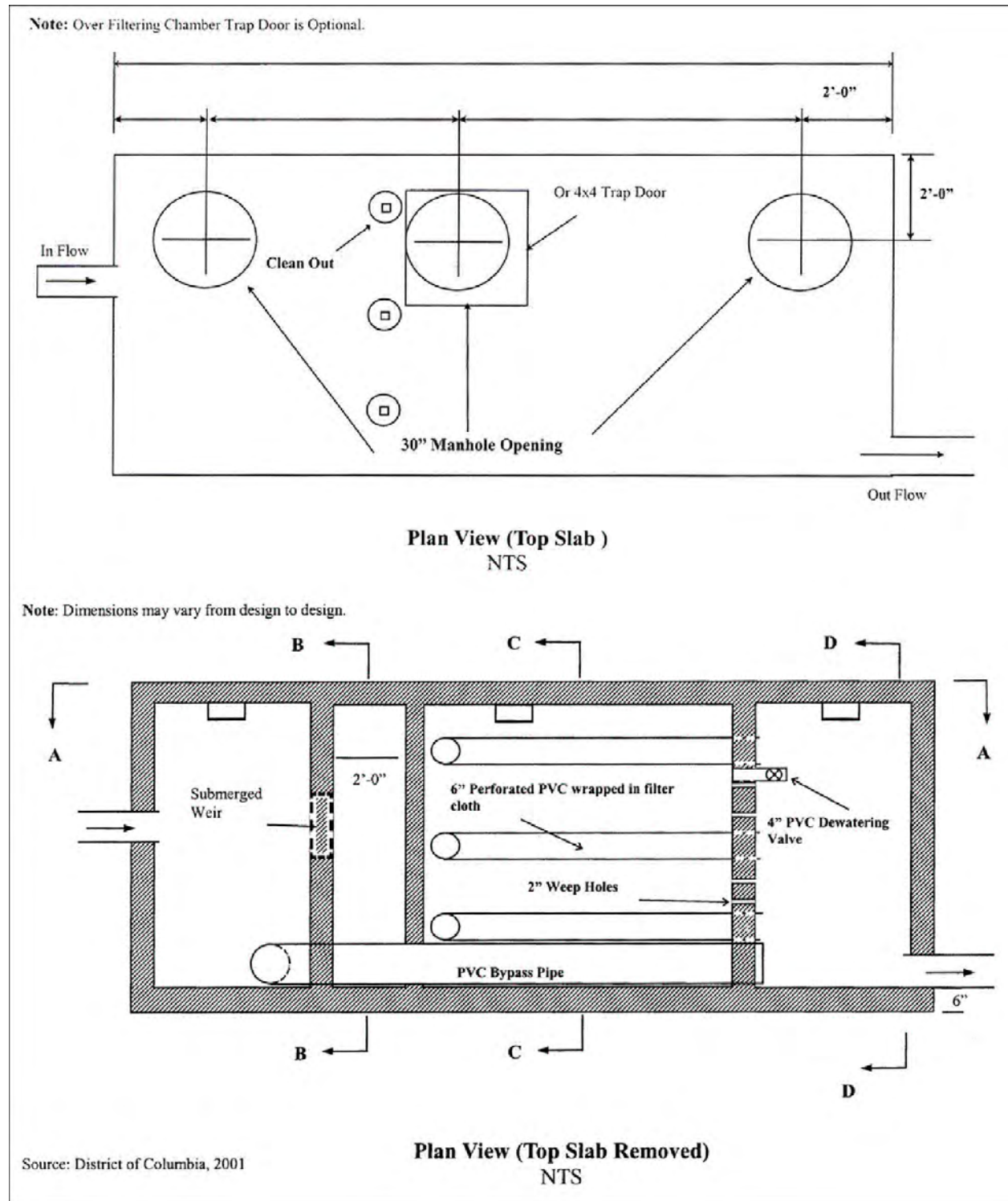
Figure 3.22 Example of a three-chamber underground sand filter (F-3) for separate sewer areas. Note: Material specifications are indicated in Table 3.28.
