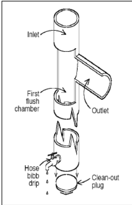
Figure 3.3 Diagram of a first flush diverter. (TWRB, 2005)
