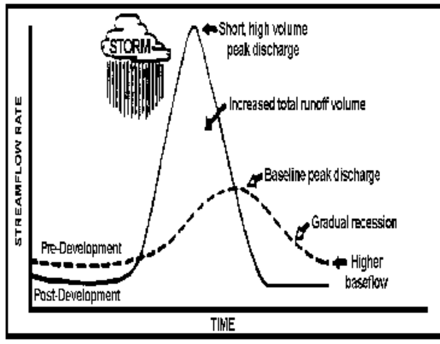
Figure 1.2 Changes in streamflow resulting from urbanization (Schueler, 1987).
