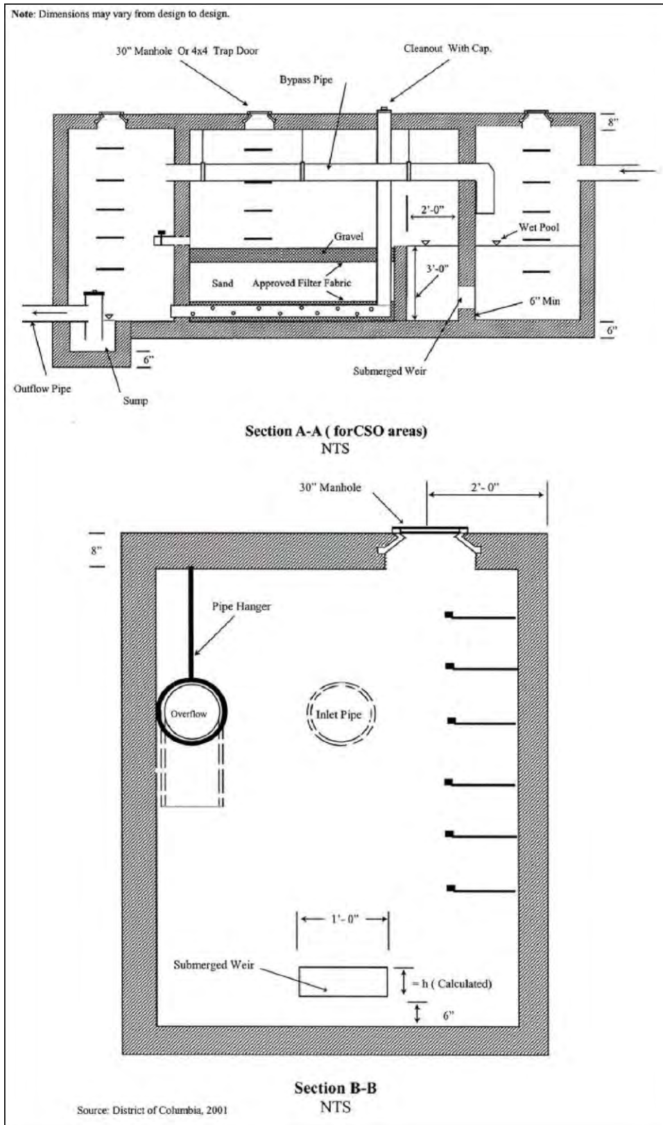
Figure 3.26 Example of a three-chamber underground sand filter (F-3) for combined sewer areas. Note: Material specifications are indicated in Table 3.28.
