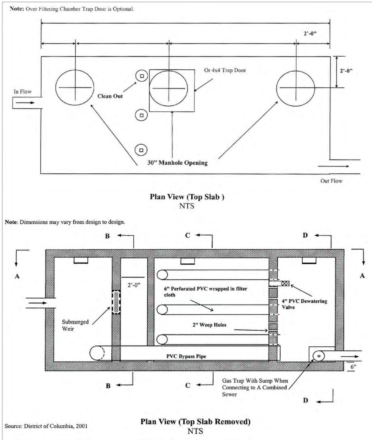
Figure 3.25 Example of a three-chamber underground sand filter (F-3) for combined sewer areas. Note: Material specifications are indicated in Table 3.28.
