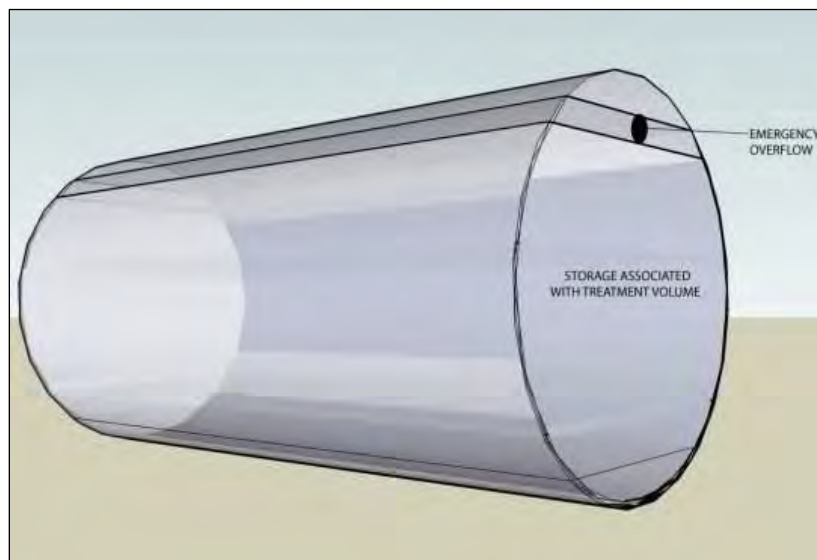
Figure 3.5 Tank Design 1: Storage associated with the design storm volume only.
