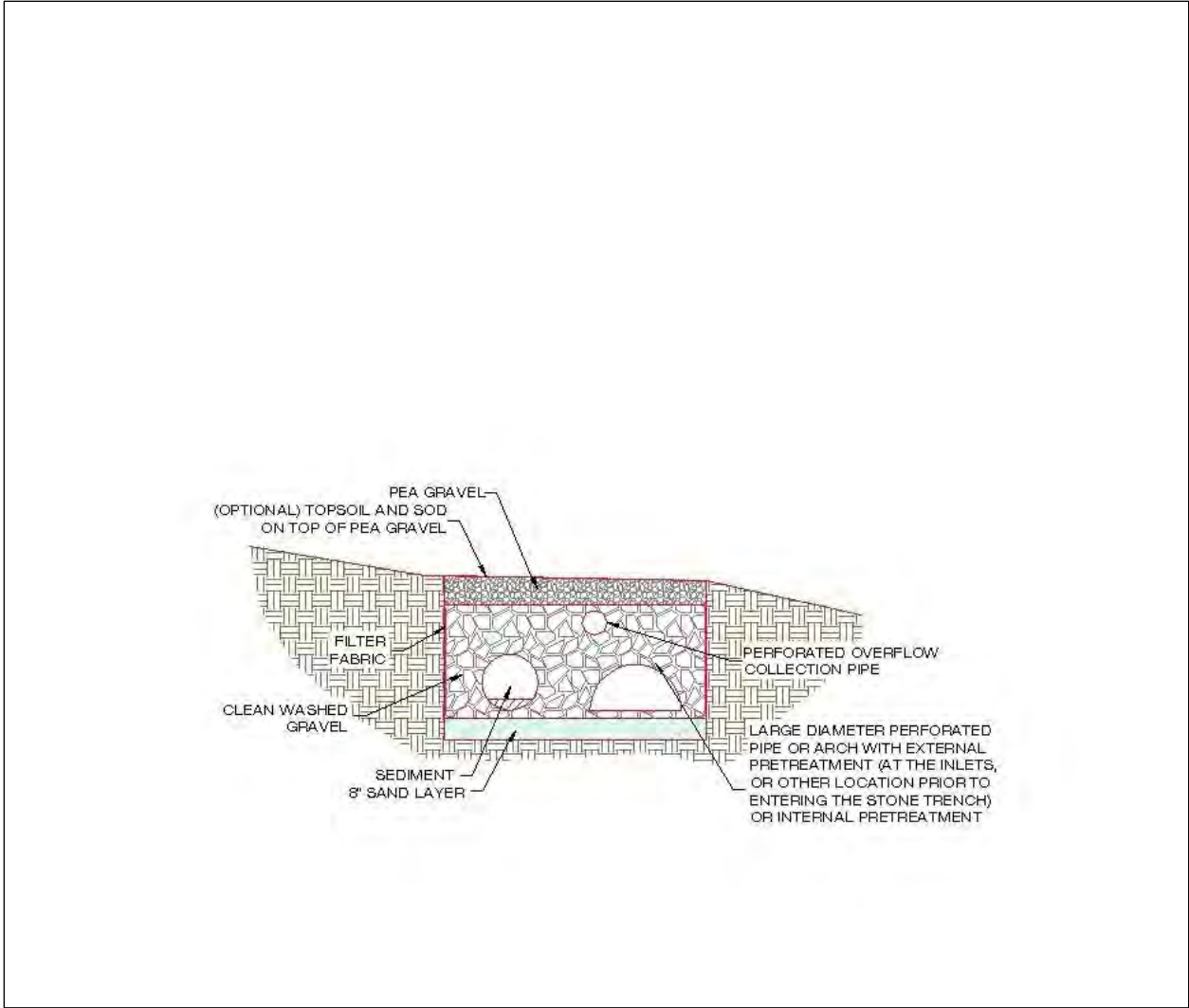
Figure 3.30 Infiltration section with supplemental pipe storage.
