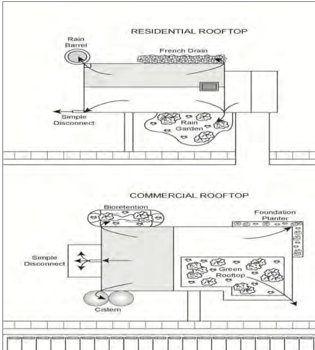
Figure 3.11 Roof disconnection with alternative retention practices
