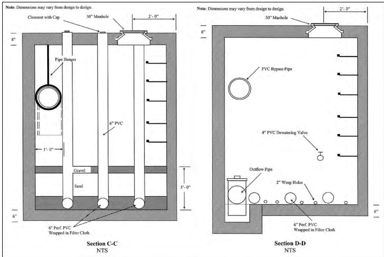
Figure 3.27 Example of a three-chamber underground sand filter (F-3) for combined sewer areas. Note: Material specifications are indicated in Table 3.28.
