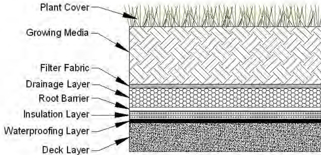
Figure 3.1 Typical layers for a green roof.
